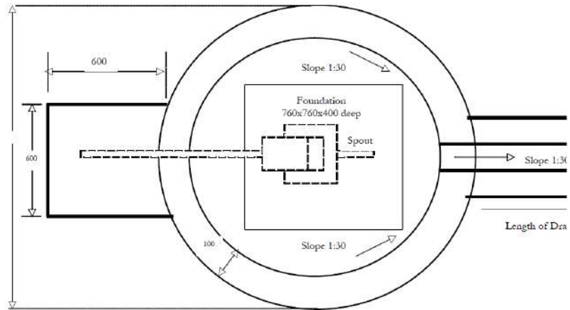
Figure 4: Drilled Well Platform Design (District Implementation Manual, 2007)
