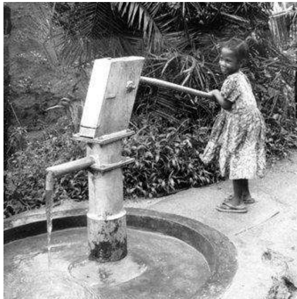
Figure 5: A U3M pump on a sealed borehole with concrete apron
