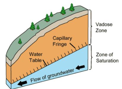
Figure 8: Illustration of the Vadose Zone (US Geological Survey)
