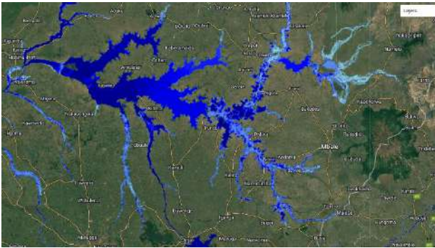
Figure 5-7: Flood depth of 100 yr ARI
