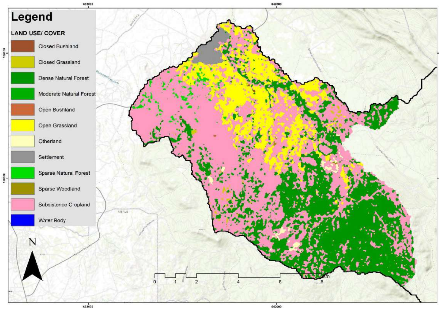
Figure 2-7: LULC cover distribution in the micro-catchment
