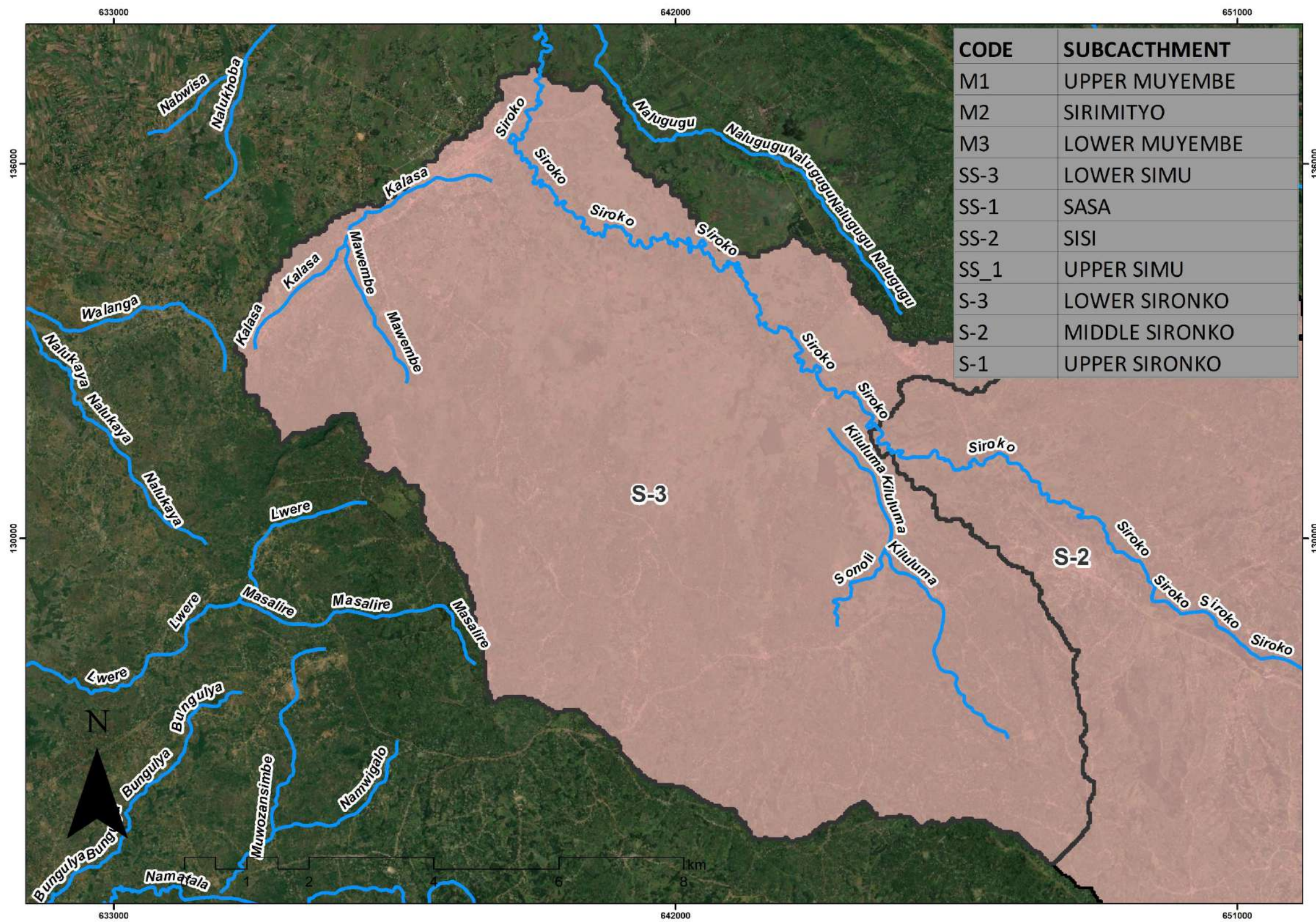
Figure 2-3: Hydrology in Lower Sironko Micro-catchment.
