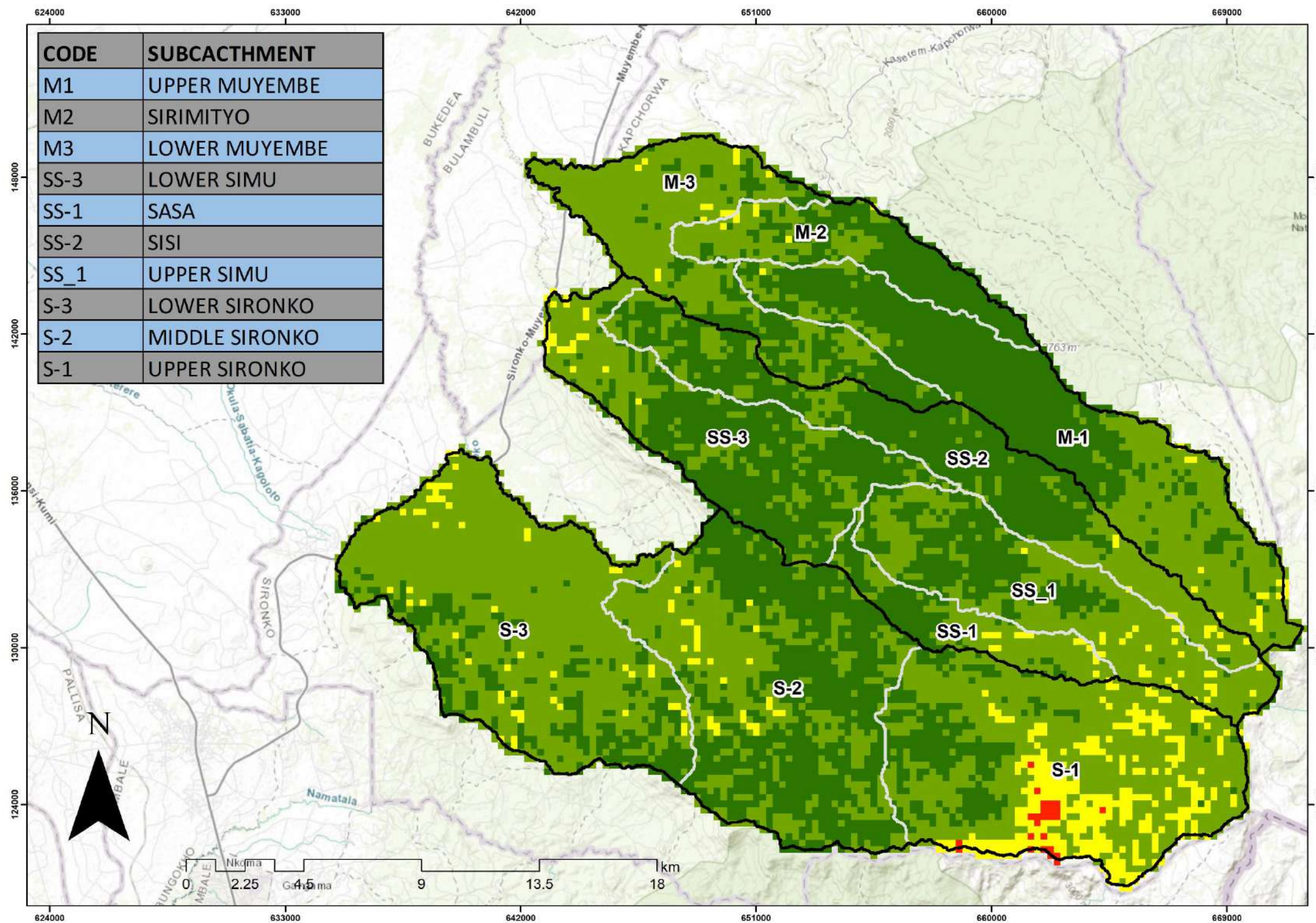
Figure 5-11: Drought distribution across Micro-catchments (See S-3)
