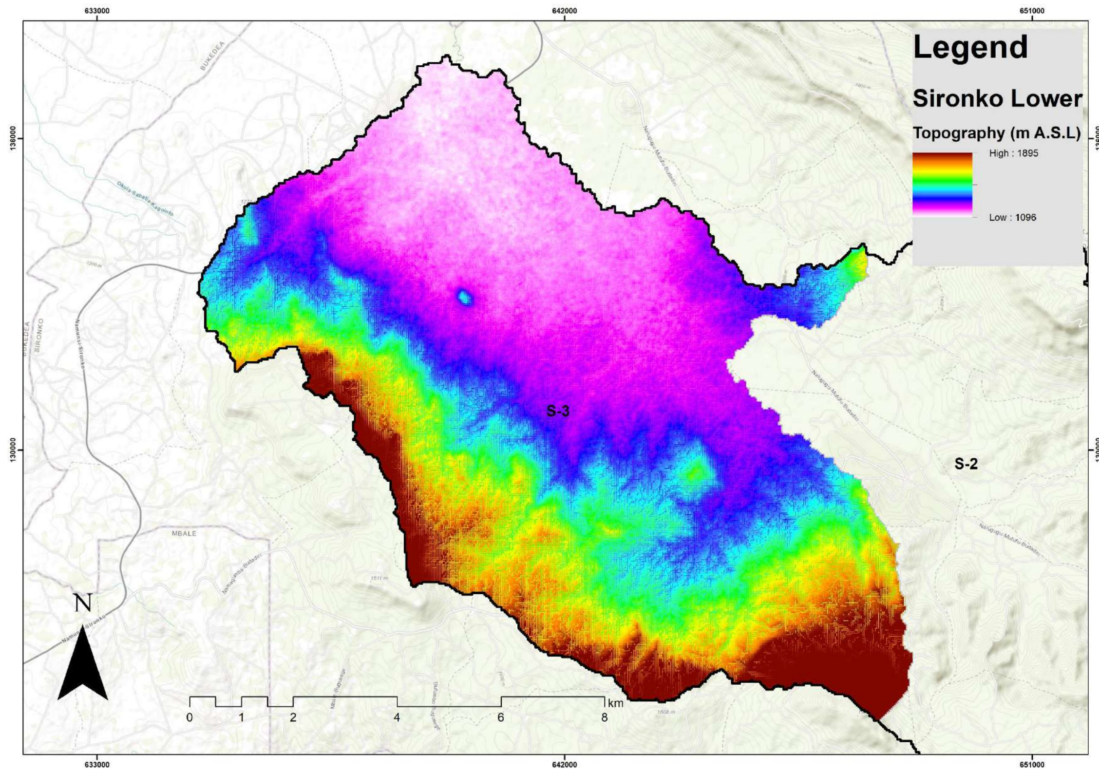
Figure 2-4: Lower Sironko Micro-catchment topography
