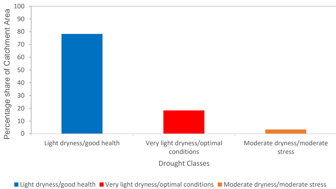
Figure 5-10: Drought class distribution across Lower Sironko micro-catchment
