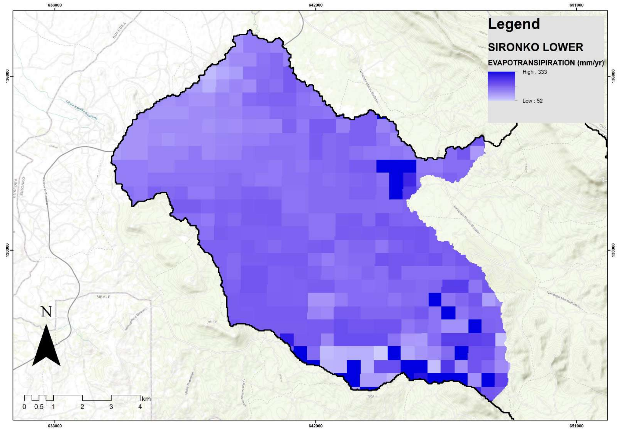
Figure 2-11: Annual Evapotranspiration distribution across the Micro-catchment.
