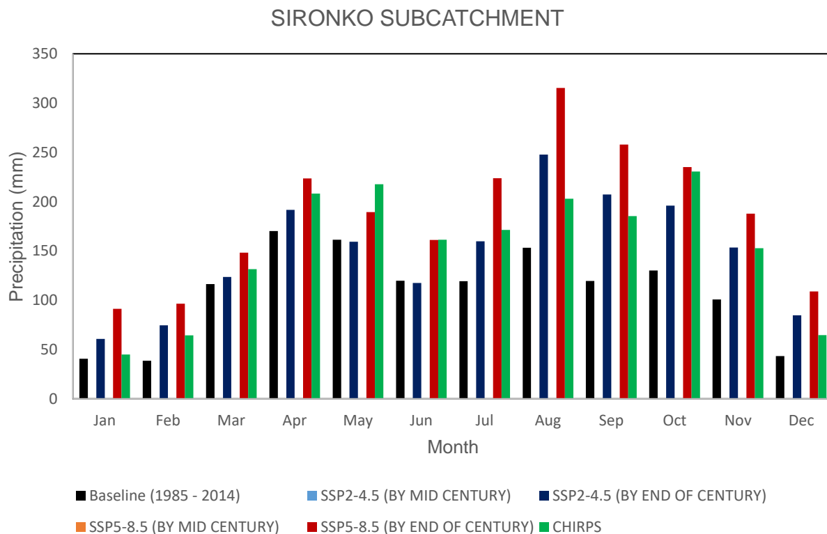
Figure 5-6: Monthly precipitation over Sironko sub-catchment based on CHIRPS, baseline (1985-2014), and for the GCM-CanESM5 projected period of 2026–2050, 2050–2100 under the SSP 2–4.5 and 5–8.5 emission scenarios
