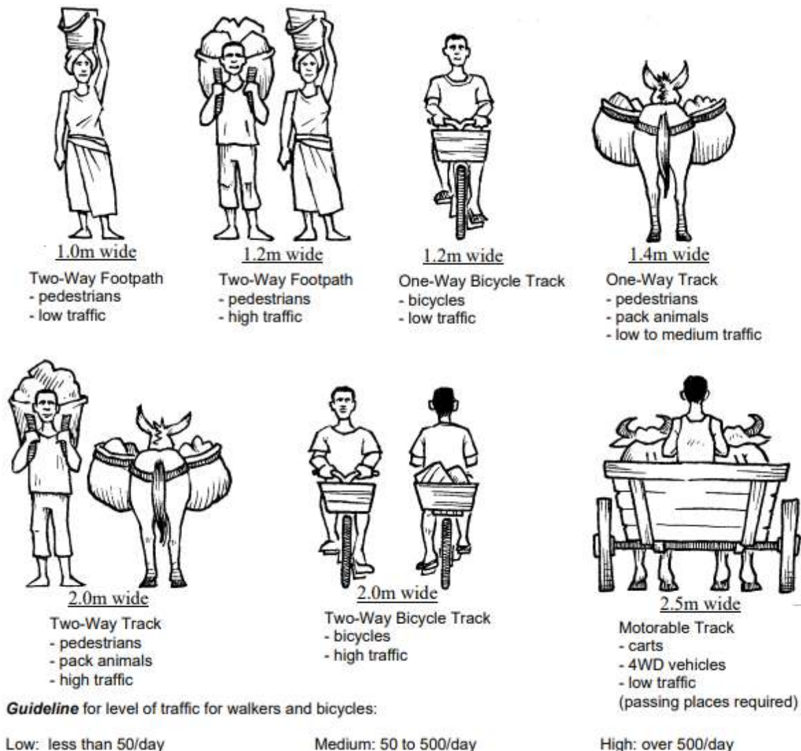
Figure 8-12: Considered standard widths for footbridges
