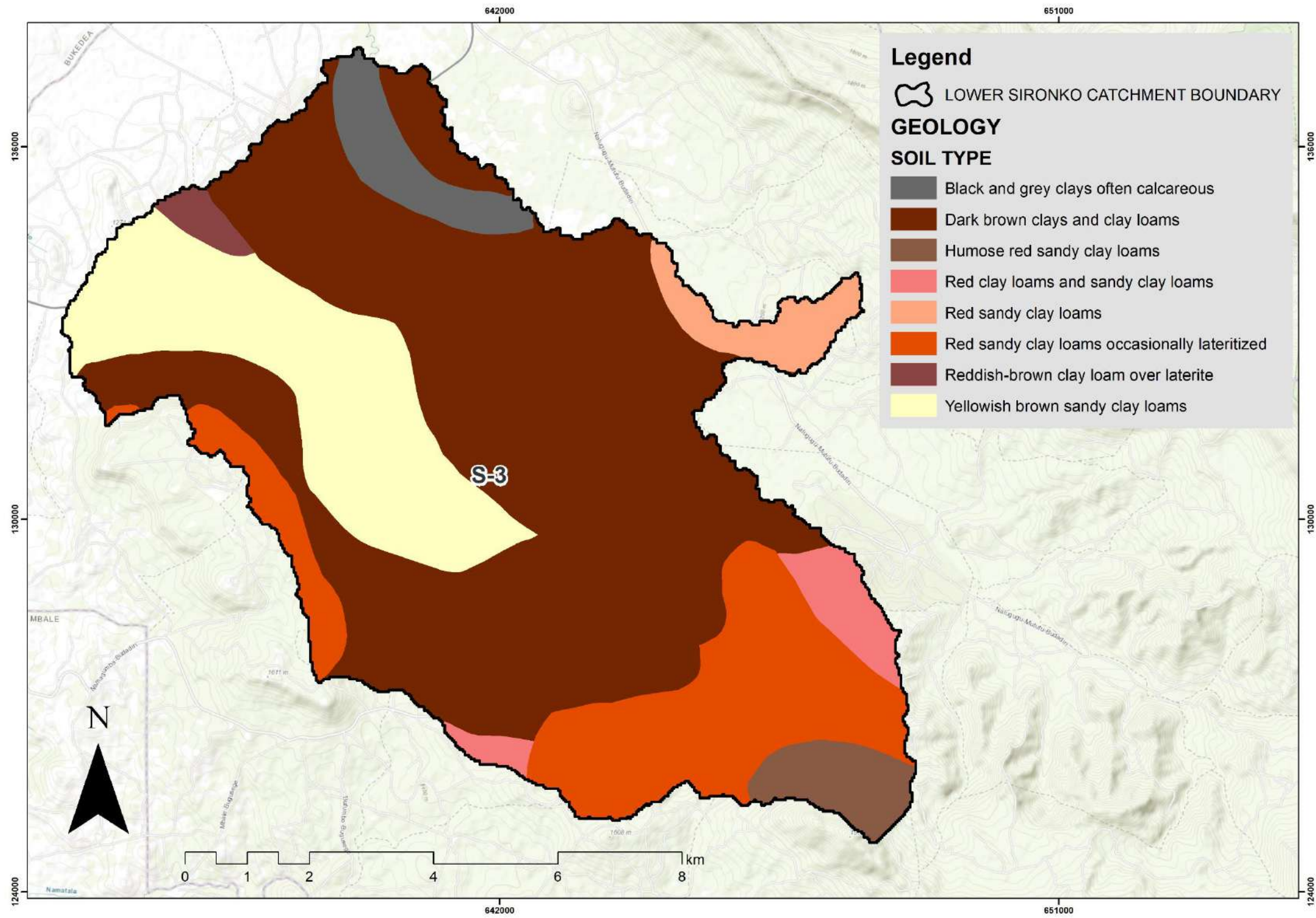
Figure 2-5: Lower Sironko Micro- catchment soil types
