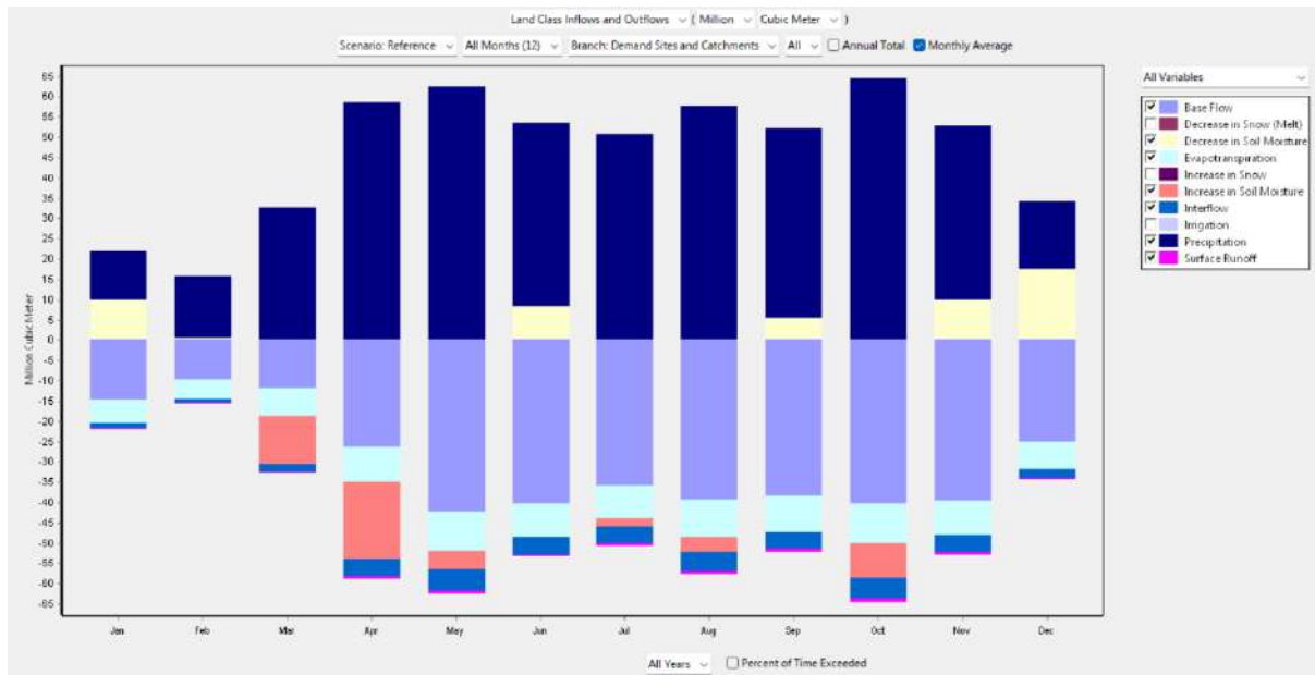
Figure 5-14: WEAP model water balance results for Sironko
