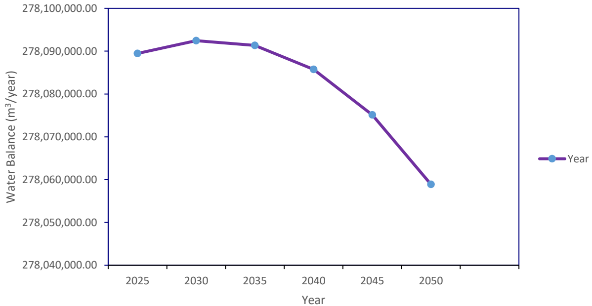
Figure 6-1: Projected water balance results for Lower Sironko micro-catchment
