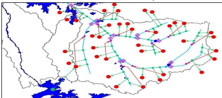
Figure 9: Schematic water resources/ demand flow in the Mpologoma catchment (Developed in WEAP)
